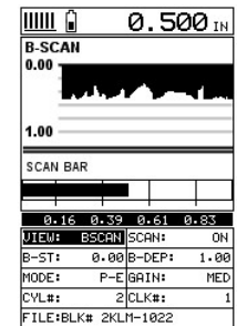
B-Scan View
